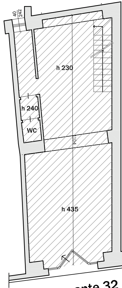
piano terra
