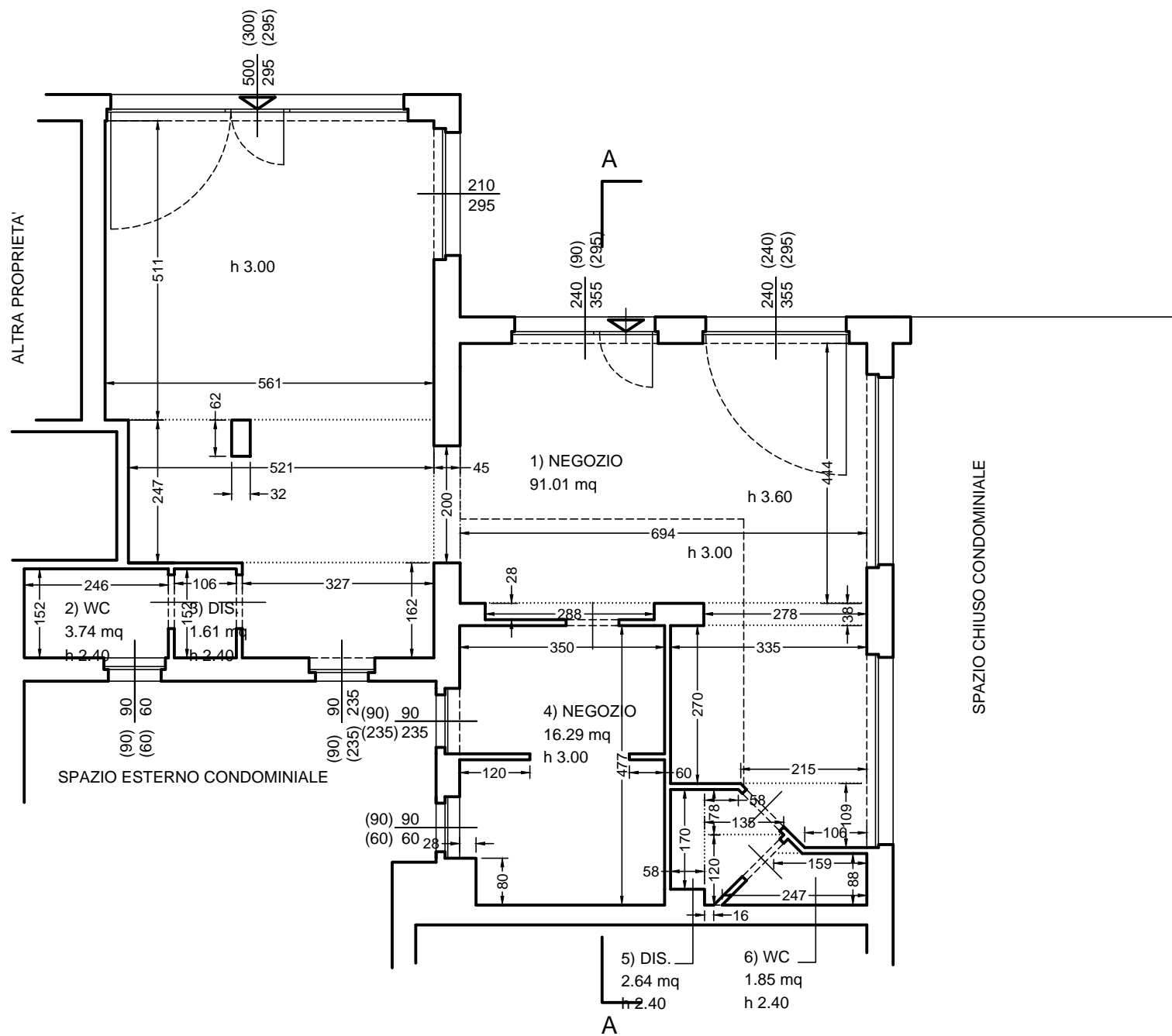
PIANO TERRA
